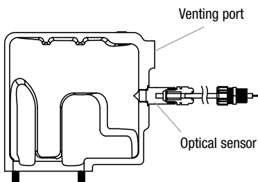
Electronic (optical) air eliminator (no moving parts)
