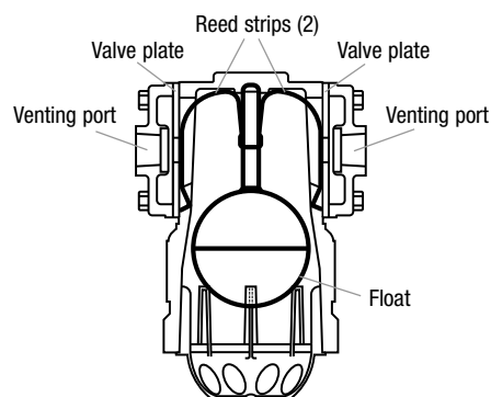
Mechanical air eliminator (float activated)
